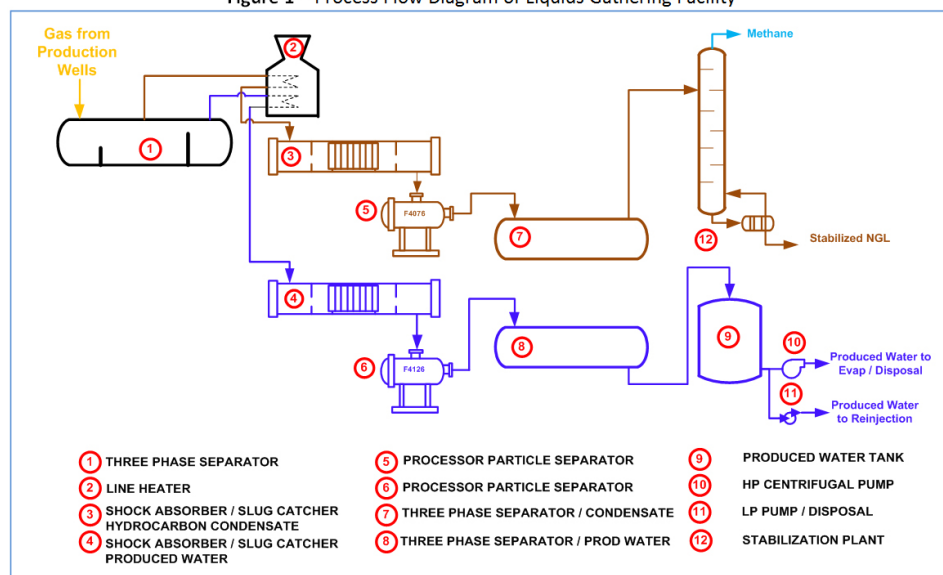
Figure 1 – Process Flow Diagram of Liquids Gathering Facility
